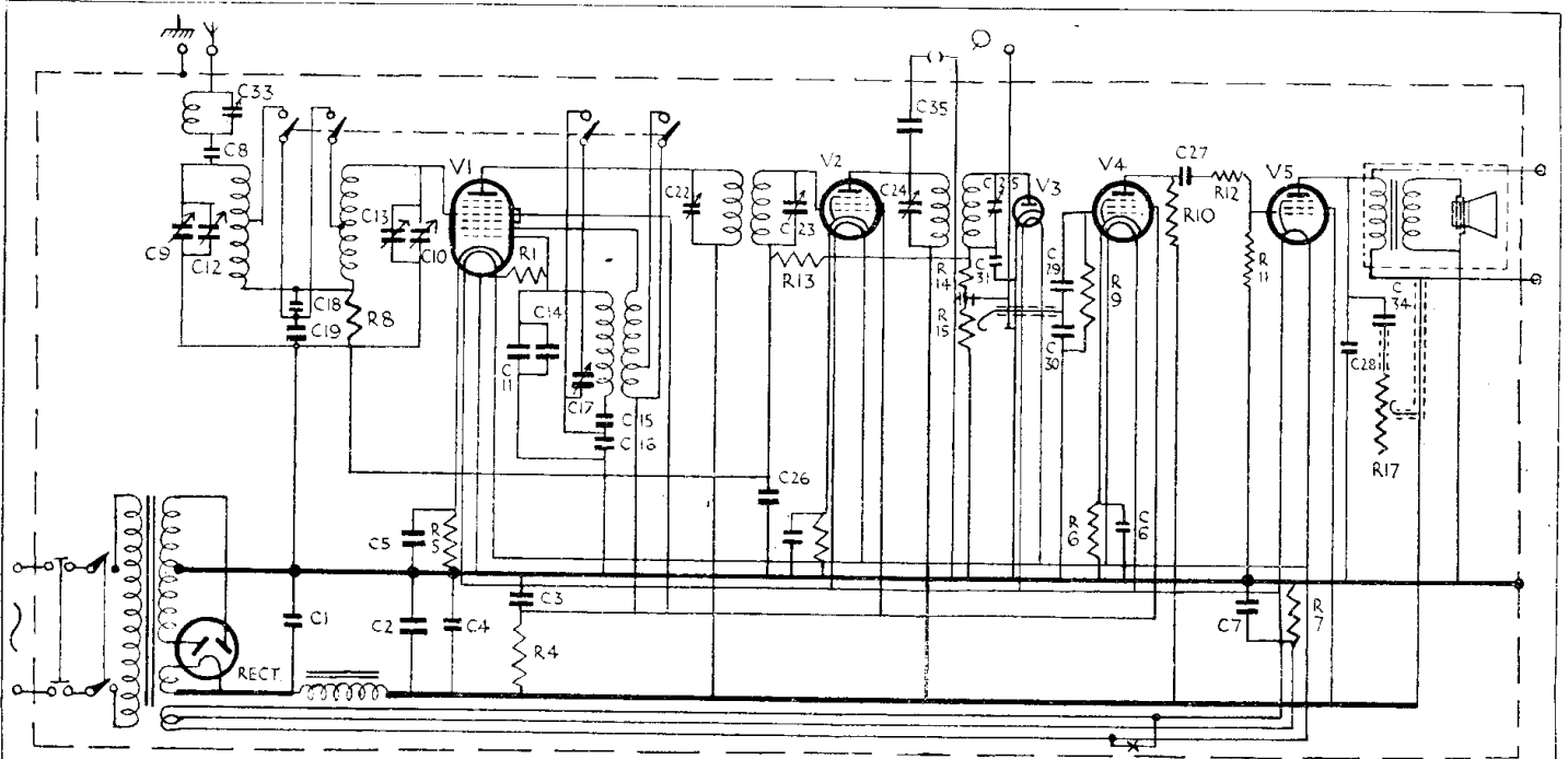
The circuit of the Philips 588A comprises an octode frequency-changer, an H.F. pentode I.F. amplifier, a diode second detector, an H.F. pentode L.F. amplifier, an output pentode and a rectifier valve.
